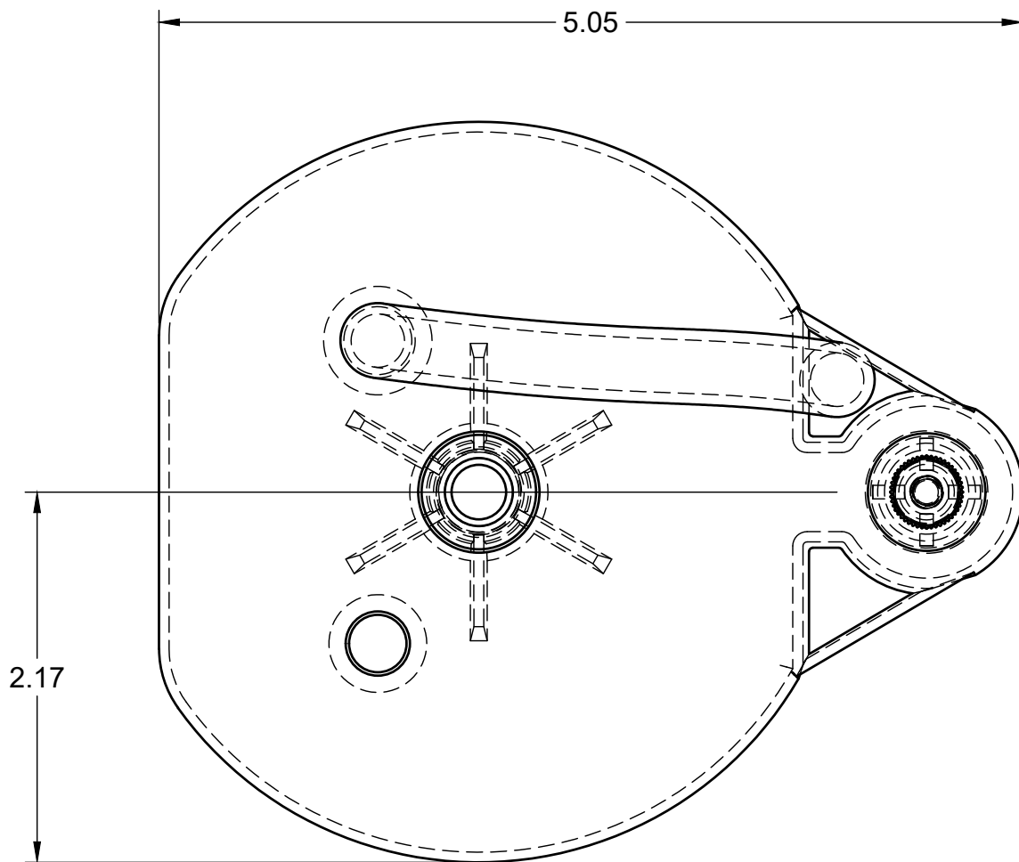
OVERFLOW PIPE INTAKE SHROUD - TOP VIEW (FULL SCALE)
