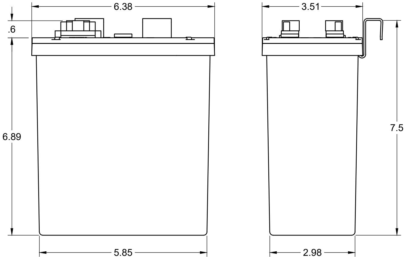
SIDE VIEW (1/2 SCALE)
