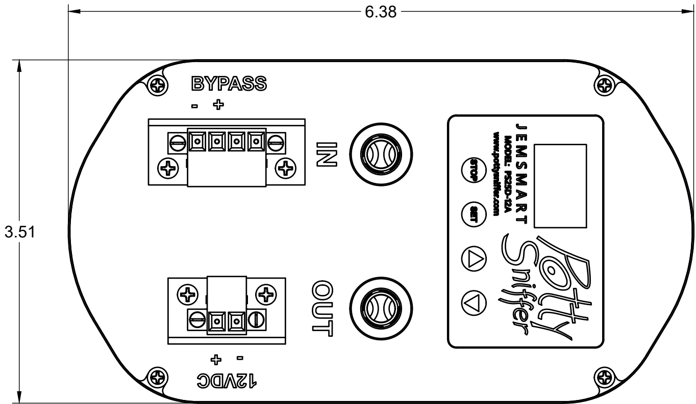
PS25D PUMP ASSY - TOP VIEW (FULL SCALE)
